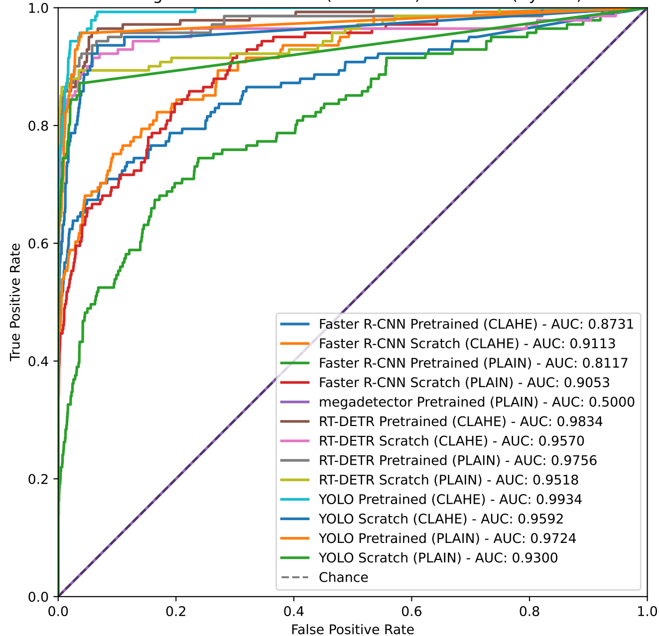
Image-Level ROC Curves (WLT Focus) - Test Pool (Cycle 0)
