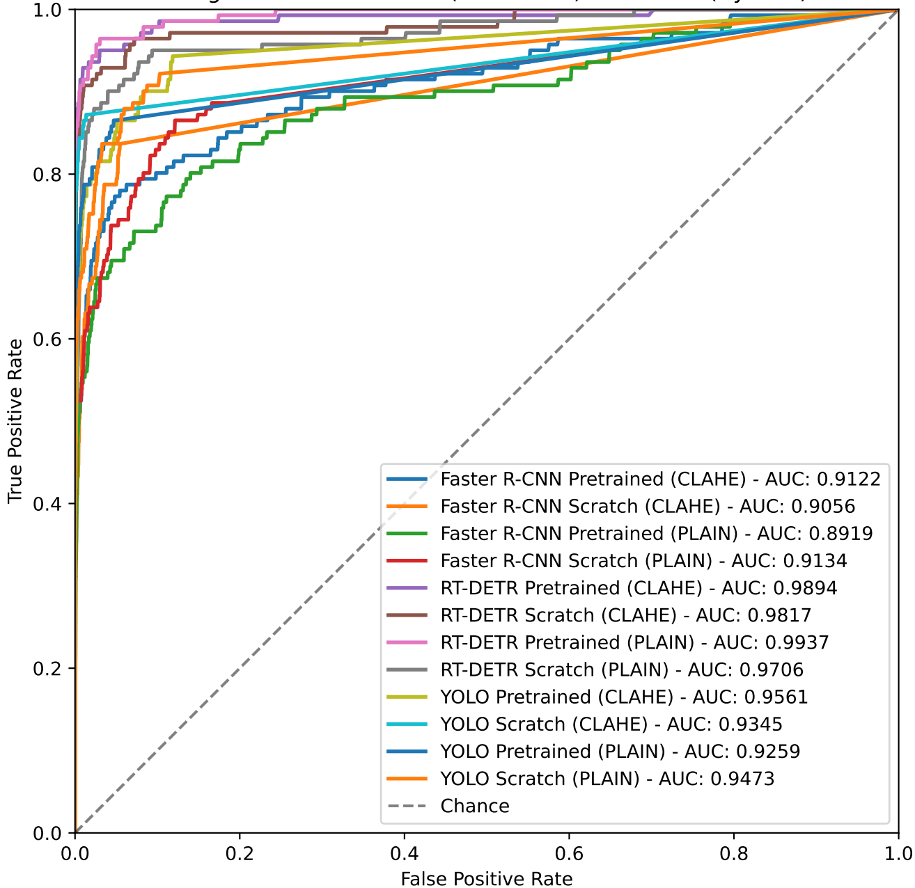
Image-Level ROC Curves (WLT Focus) - Test Pool (Cycle 3)
