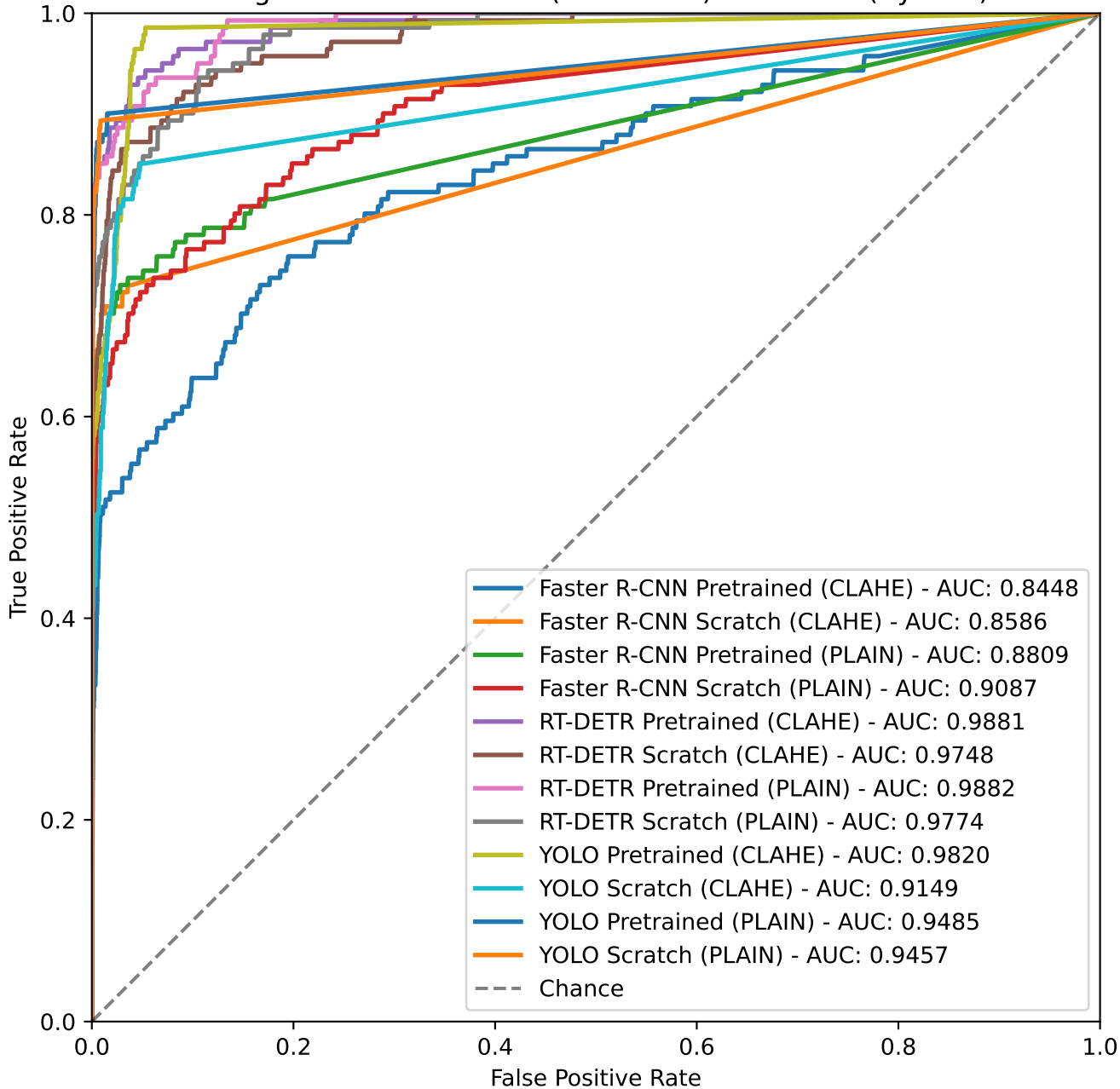
Image-Level ROC Curves (WLT Focus) - Test Pool (Cycle 4)
