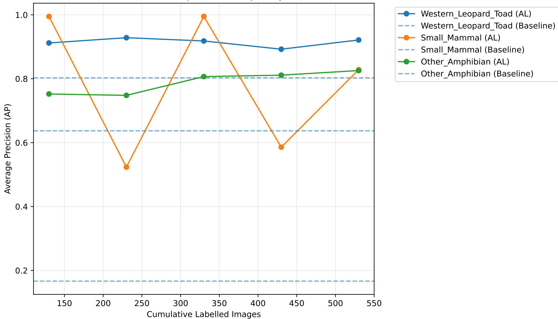
YOLO Class-Specific AP Trajectory
