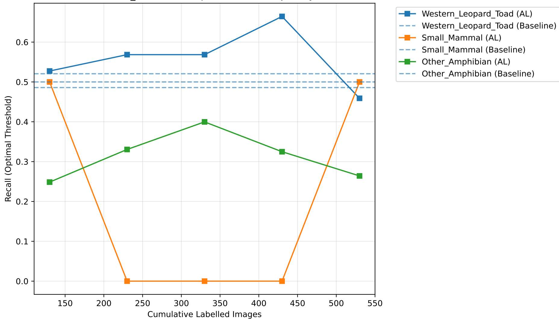
FASTER_RCNN Class-Specific Recall Trajectory
