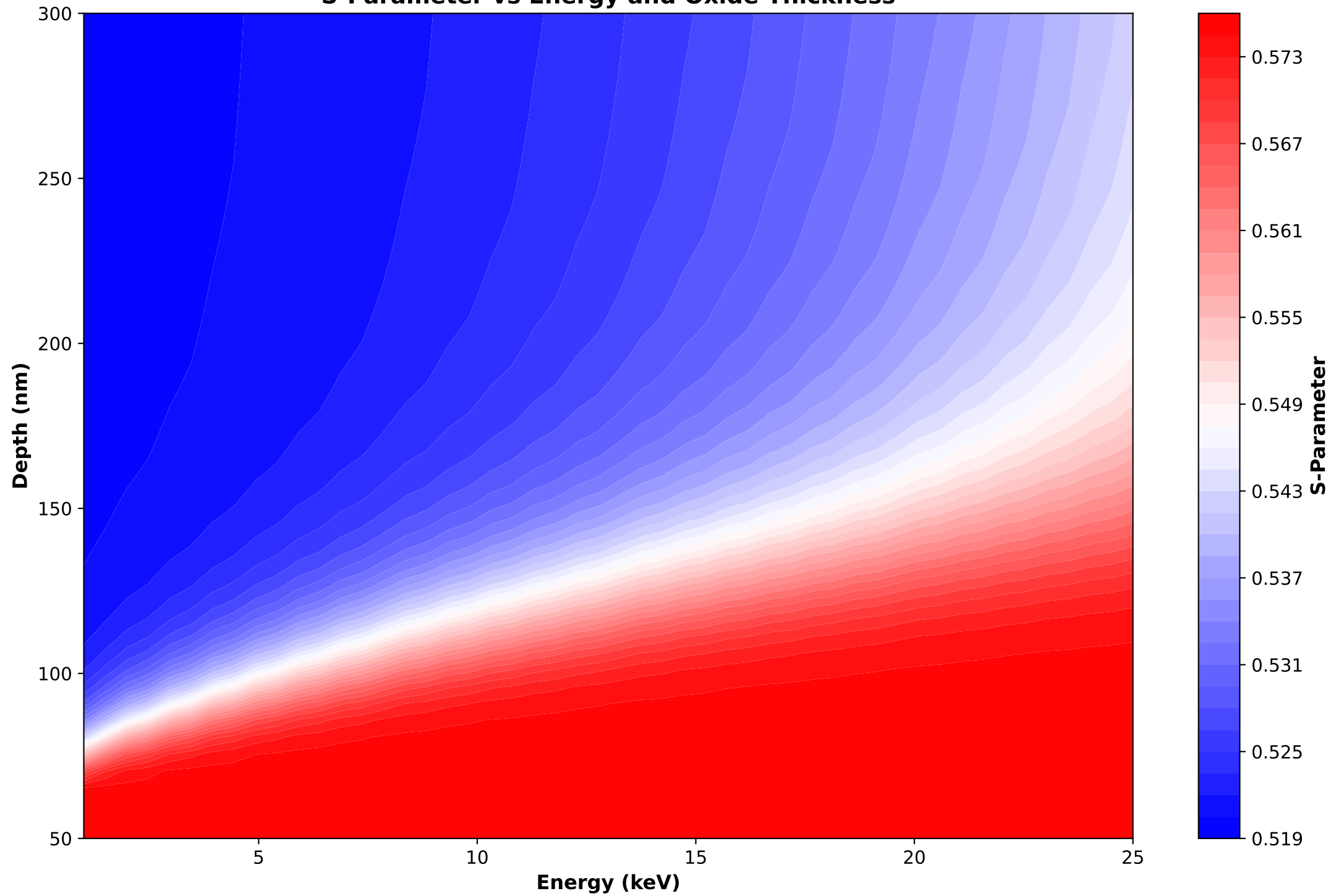
S-Parameter vs Energy and Oxide Thickness
