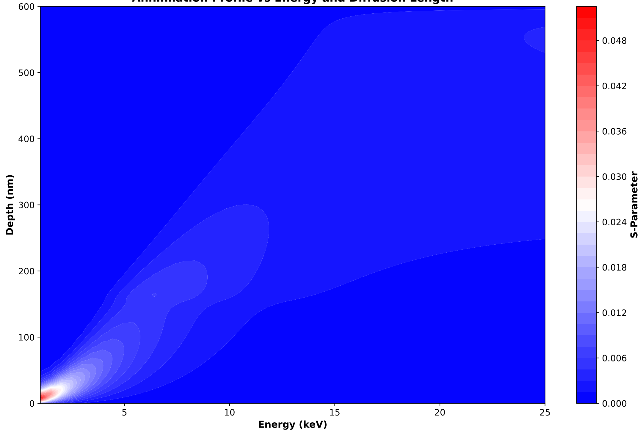
Annihilation Profile vs Energy and Diffusion Length
