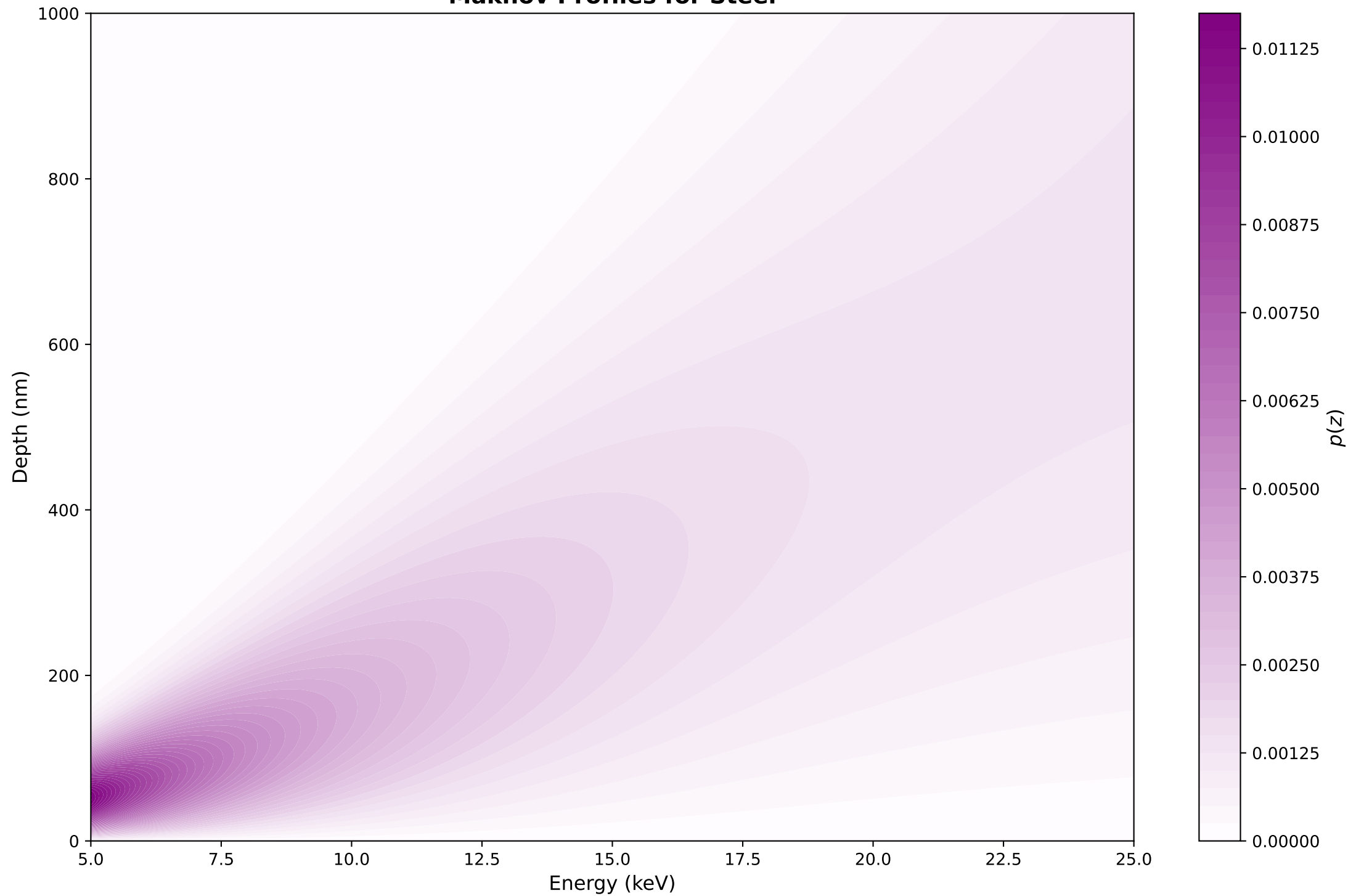
Makhov Profiles for Steel
