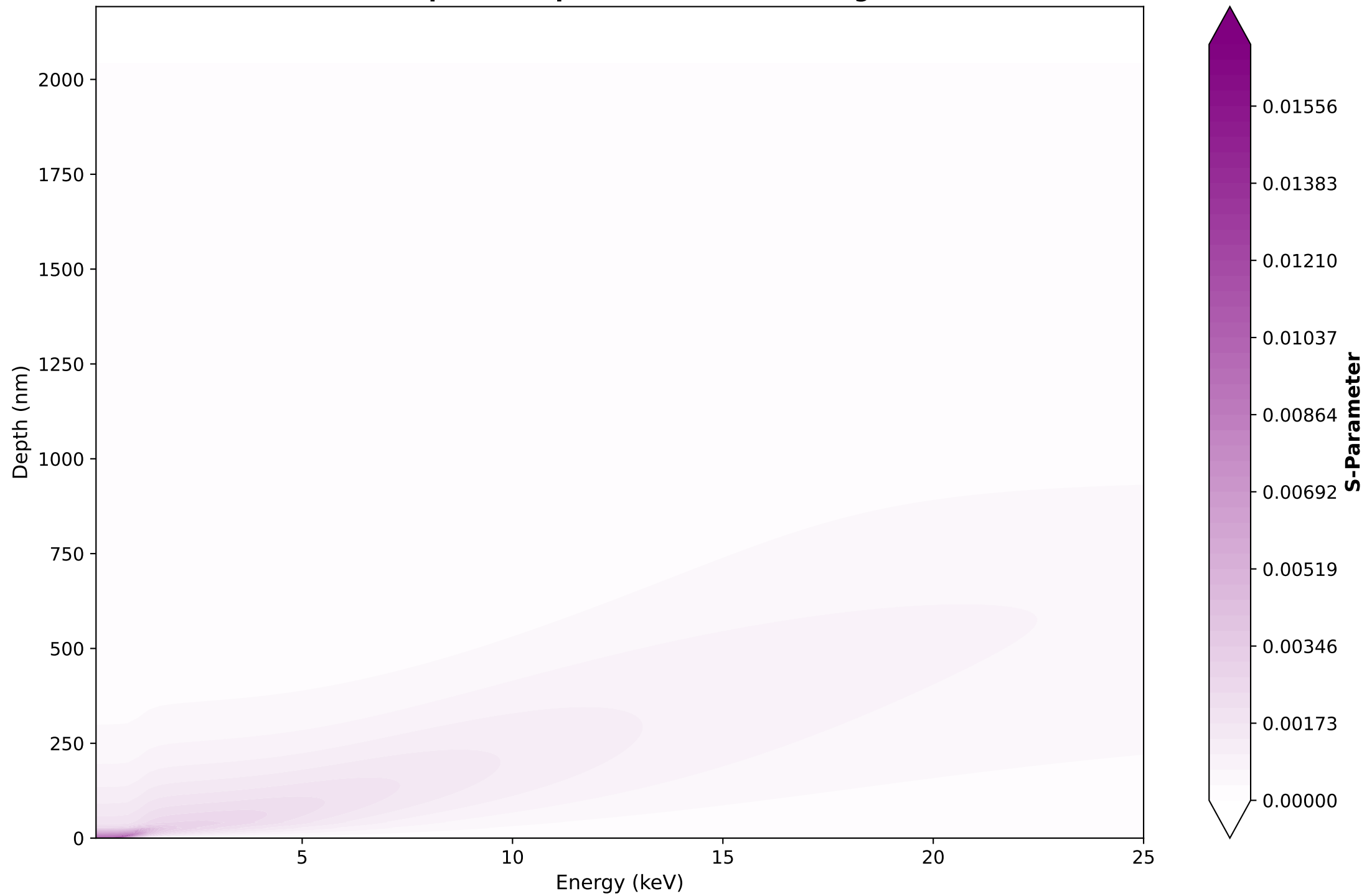
Overlap Heatmap (30.0% Oxide Coverage)
