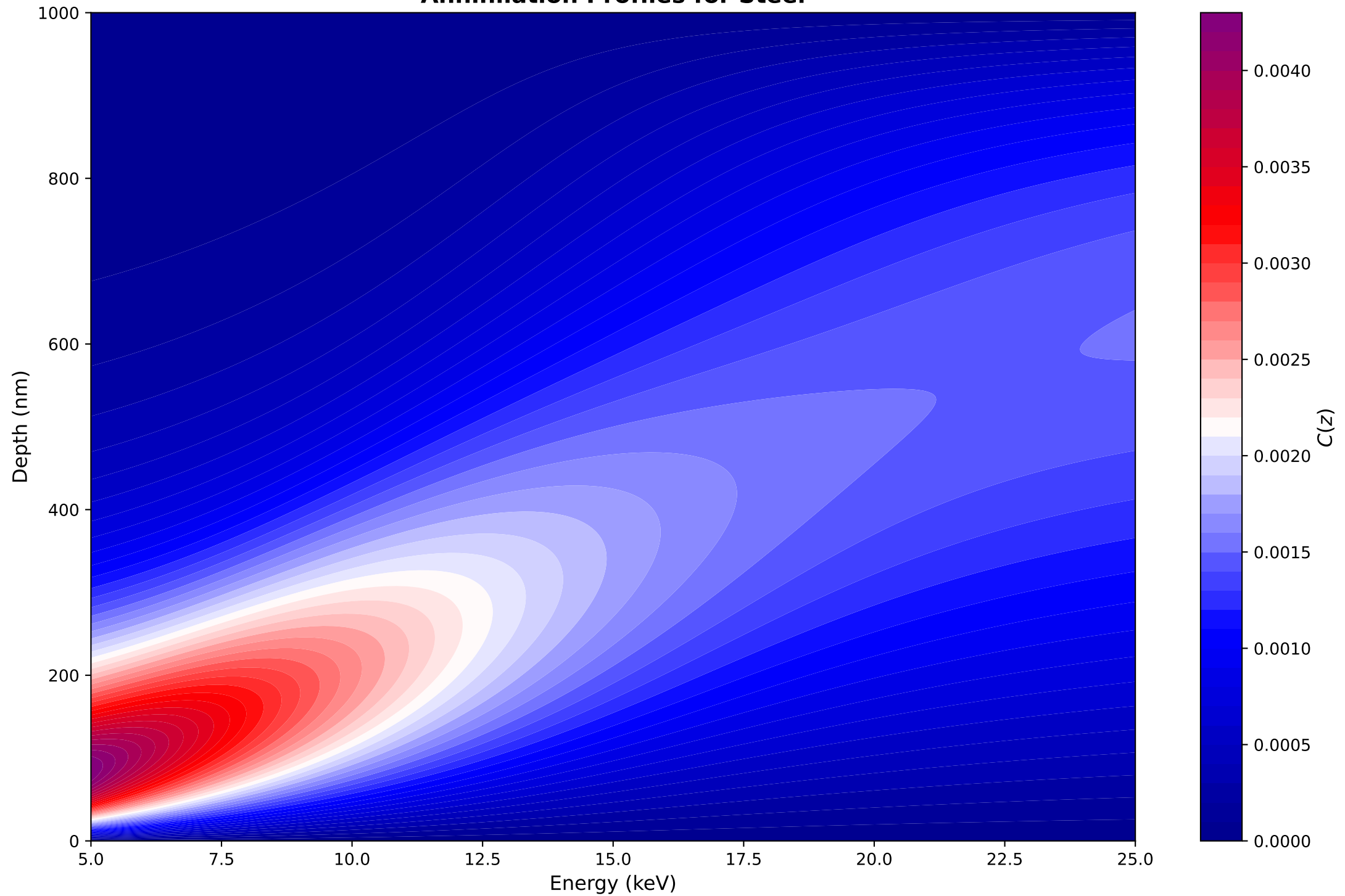
Annihilation Profiles for Steel
