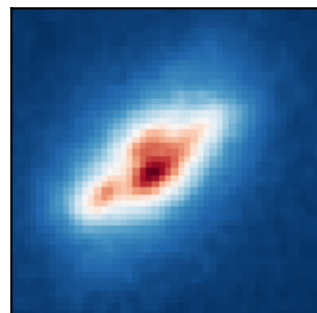
ground truth
