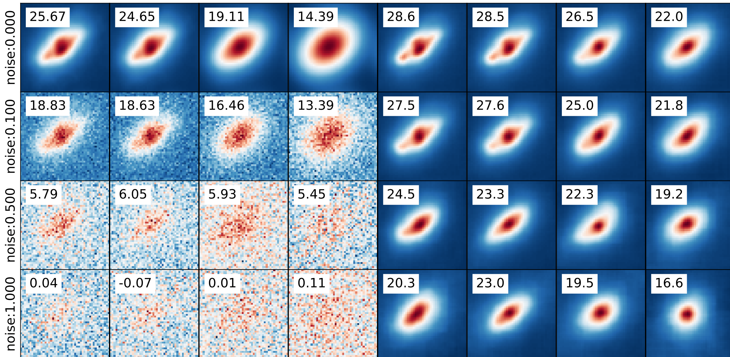
ground truth
