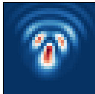
PSF optics
