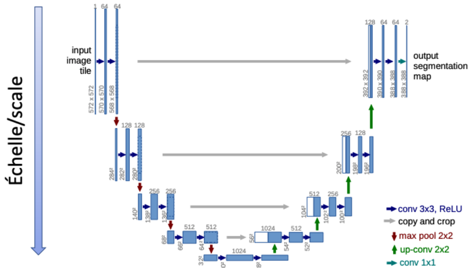
FIGURE 34 – Architecture multi-échelles d’un U-Net.
