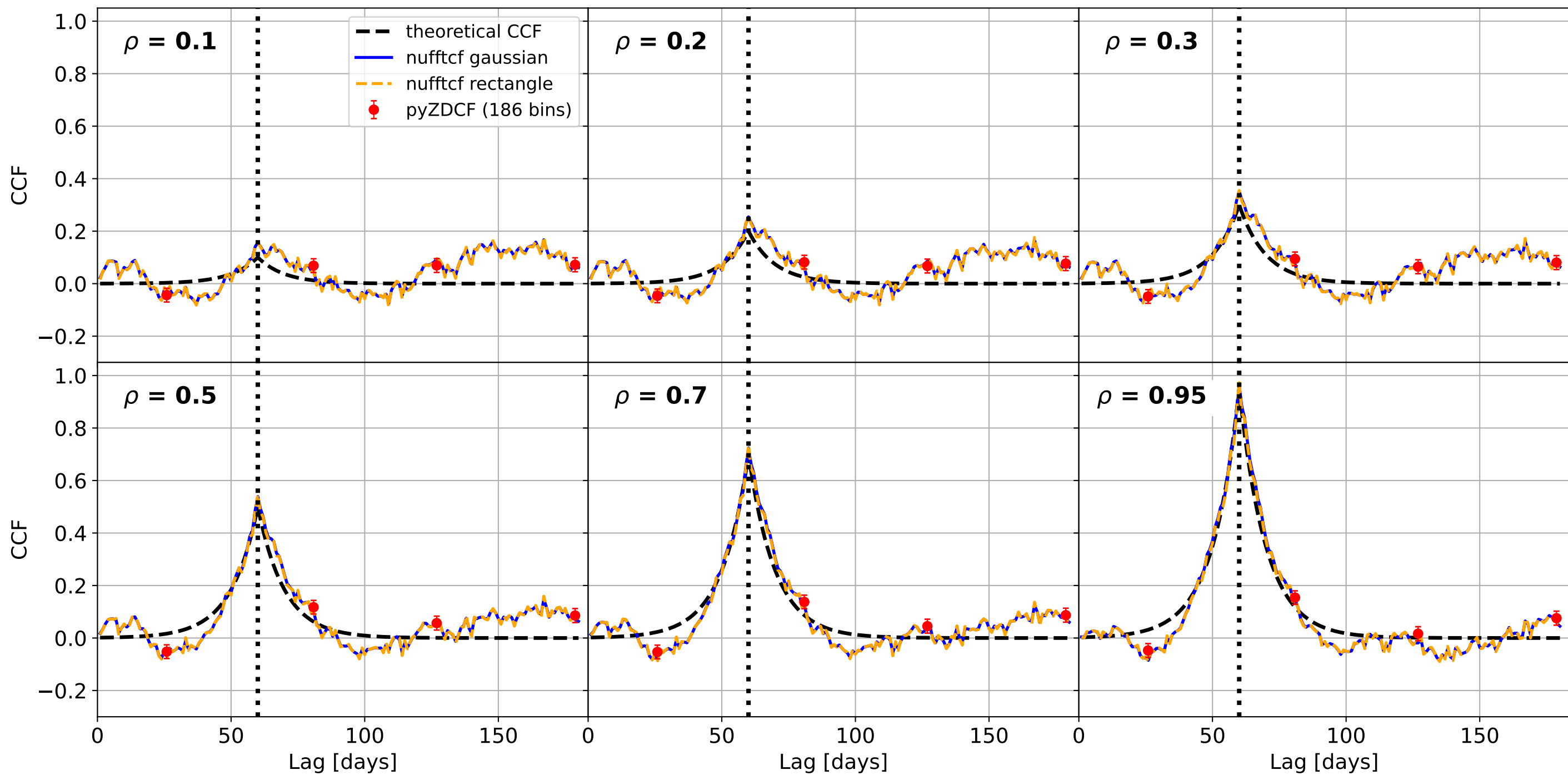
CCF of coupled Ornstein-Uhlenbeck processes ( \tau_0=60 d, \alpha=10.0 )
