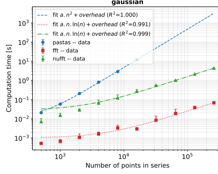
Figure 9: ACF benchmark on regularly-sampled data, pastas versus nufftcf (dedicated FFT path and general-purpose NUFFT path), gaussian kernel.
