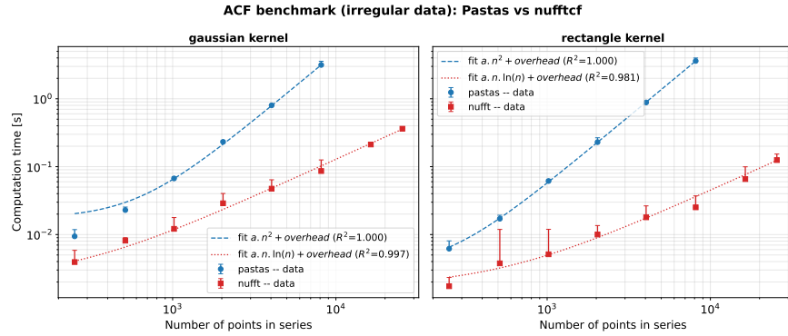
Figure 8: ACF benchmark, nufftcf versus pastas , on irregularly-sampled data (gaussian and rectangle kernels). Robust fit (soft_l1); error bars show the min-to-max spread across repeats at each point.
