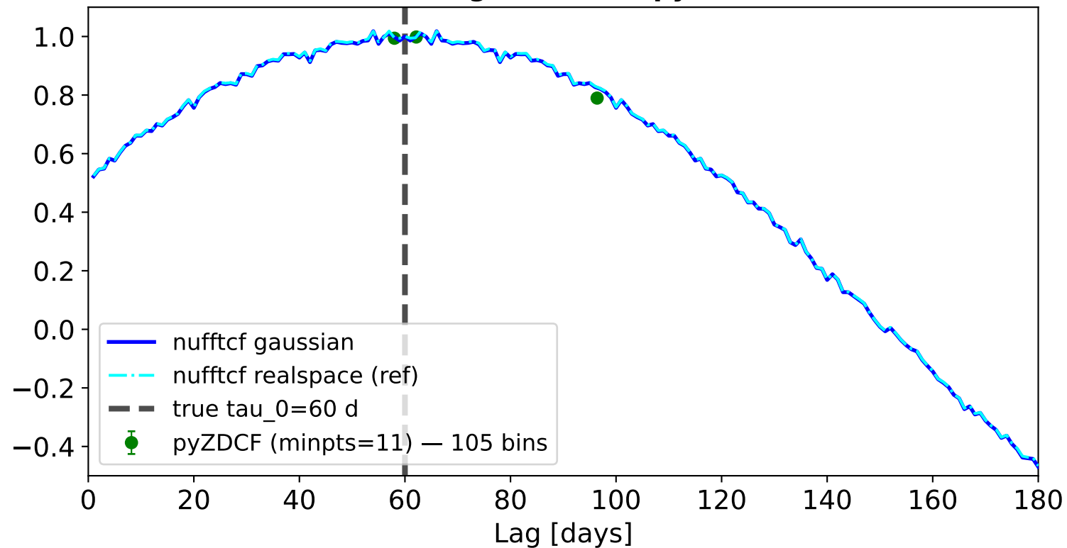
nufftcf gaussian vs pyZDCF
