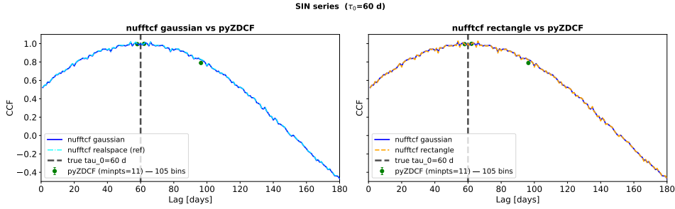
FIG. 6.— CCF of the shifted-timestamp SIN network test ( \tau_0 = 60 d): nufftcf Gaussian vs. its own real-space reference (left) and vs. its rectangular kernel (right), both compared to pyZDCF .
