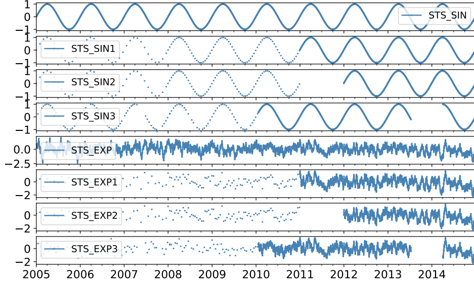
FIG. 1.— The eight synthetic series used in the ACF benchmark: the fully-sampled reference processes (STS_SIN, STS_EXP) and their three irregularly-sampled derivatives each (STS_SIN1–3, STS_EXP1–3), reproduced from the pastas autocorrelation-benchmark tutorial.
