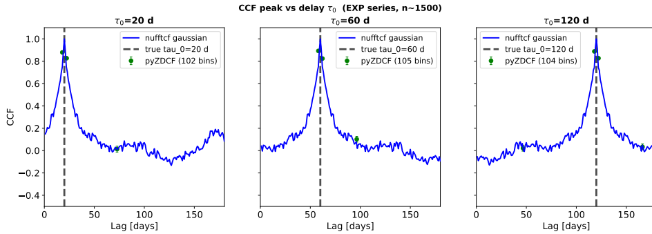
FIG. 8.— CCF peak recovery for the shifted-timestamp EXP network test as the injected delay \tau_0 varies over \{20, 60, 120\} d ( n \sim 1500 points per network): nufftcf Gaussian vs. pyZDCF , with the true delay marked by the vertical dashed line.
