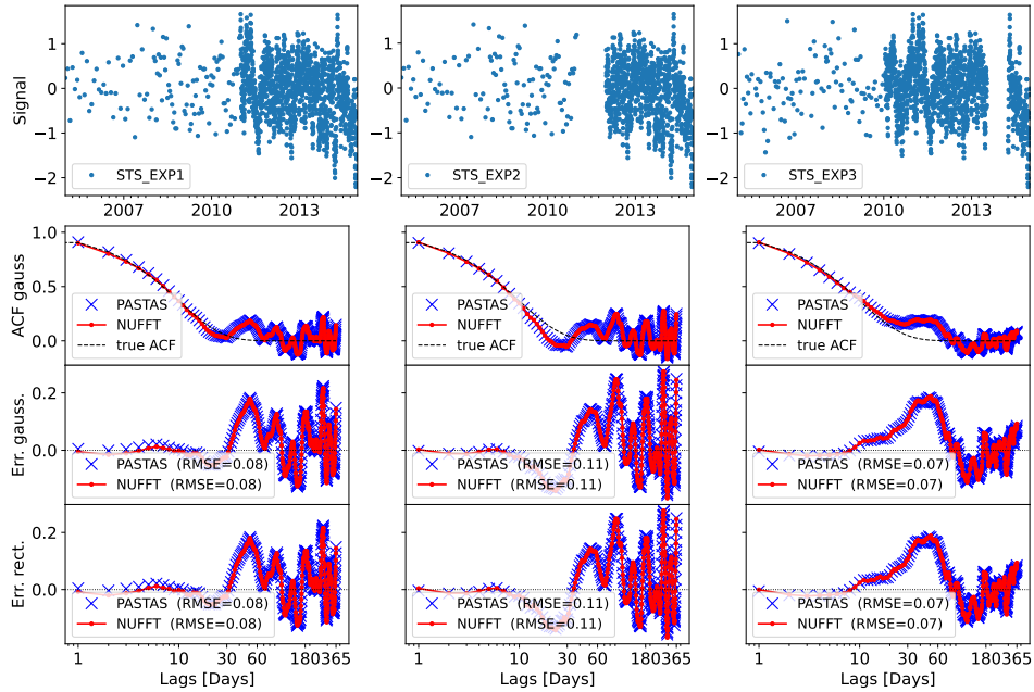
FIG. 2.— ACF of the STS_EXP1–3 series: signal (top row), pastas vs. nufftcf Gaussian-kernel ACF against the analytical truth (second row), and residuals for the Gaussian and rectangular kernels (third and fourth rows), with matching RMSE values for both estimators in every panel.
