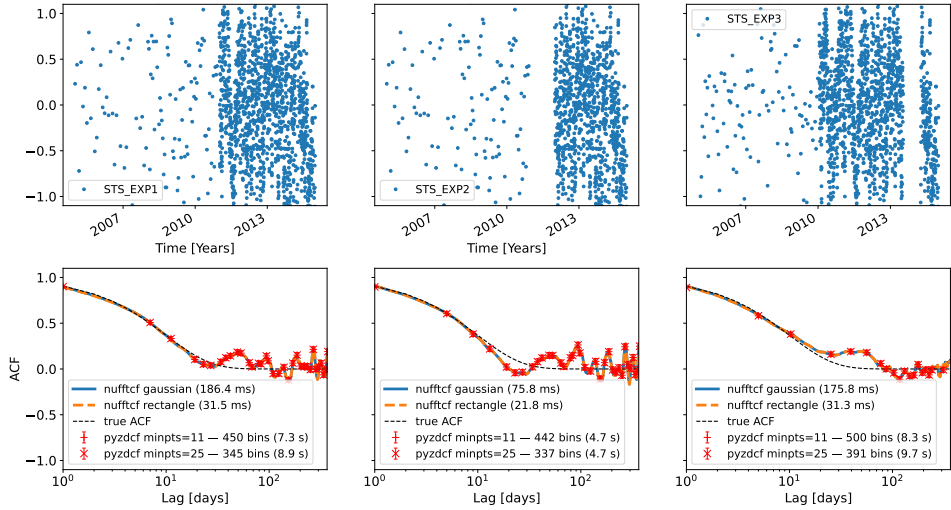
FIG. 4.— ACF of the STS_EXP1–3 series: signal (top row) and ACF (bottom row), comparing nufftcf (Gaussian and rectangular kernels, with per-series computation time) to pyZDCF ( minpts =11 and 25, with number of returned bins and computation time) and to the analytical truth.
