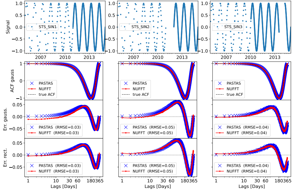
FIG. 3.— Same as Figure 2, for the STS_SIN1–3 series.
