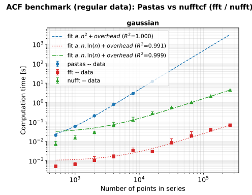
Figure 9: ACF benchmark on regularly-sampled data, pastas versus nufftcf (dedicated FFT path and general-purpose NUFFT path), gaussian kernel.
