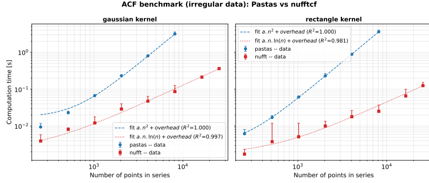
Figure 8: ACF benchmark, nufftcf versus pastas , on irregularly-sampled data (gaussian and rectangle kernels). Robust fit ( soft_l1 ); error bars show the min-to-max spread across repeats at each point.
