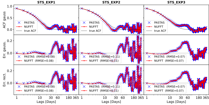
Figure 3: Same as Figure 2, for the STS_EXP1–3 series.
