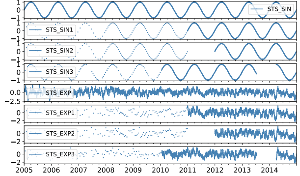
Figure 1: The synthetic series used in the ACF benchmark: the fully-sampled reference processes (STS_SIN, STS_EXP) and their three irregularly-sampled derivatives each (STS_SIN1–3, STS_EXP1–3), reproduced from the pastas autocorrelation-benchmark tutorial.
