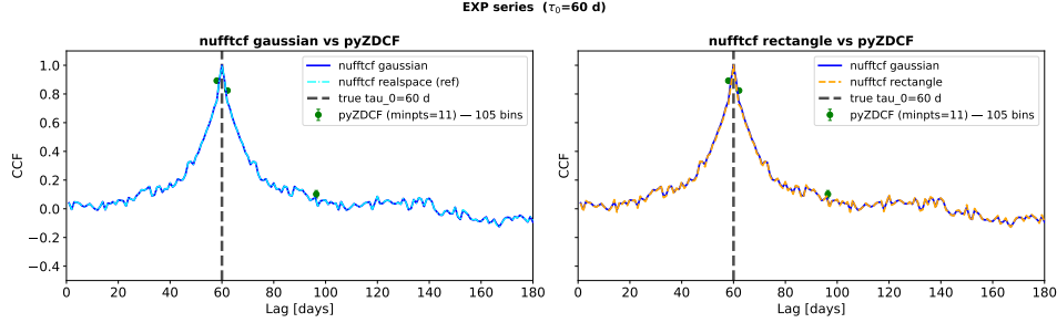
FIG. 6.— Same as Figure 5, for the shifted-timestamp EXP network test.
