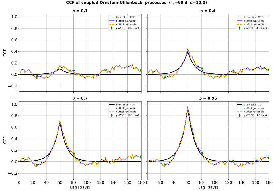
FIG. 8.— CCF of the coupled Ornstein-Uhlenbeck processes of Equation 8 ( \tau_0 = 60 d, \alpha = 10 d), for coupling strengths \rho = 0.1, 0.4, 0.7, 0.95 : nufftcf (Gaussian and rectangular kernels) and pyZDCF against the analytical CCF of Equation 9.
