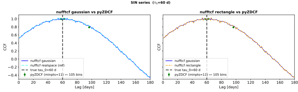
FIG. 5.— CCF of the shifted-timestamp SIN network test ( \tau_0 = 60 d): nufftcf Gaussian vs. its own real-space reference (left) and vs. its rectangular kernel (right), both compared to pyZDCF .
