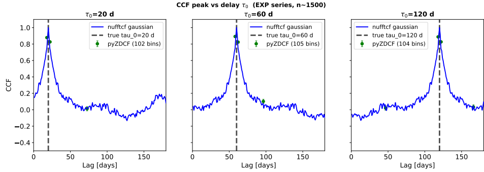
FIG. 7.— CCF peak recovery for the shifted-timestamp EXP network test as the injected delay \tau_0 varies over \{20, 60, 120\} d ( n \sim 1500 points per network): nufftcf Gaussian vs. pyZDCF , with the true delay marked by the vertical dashed line.
