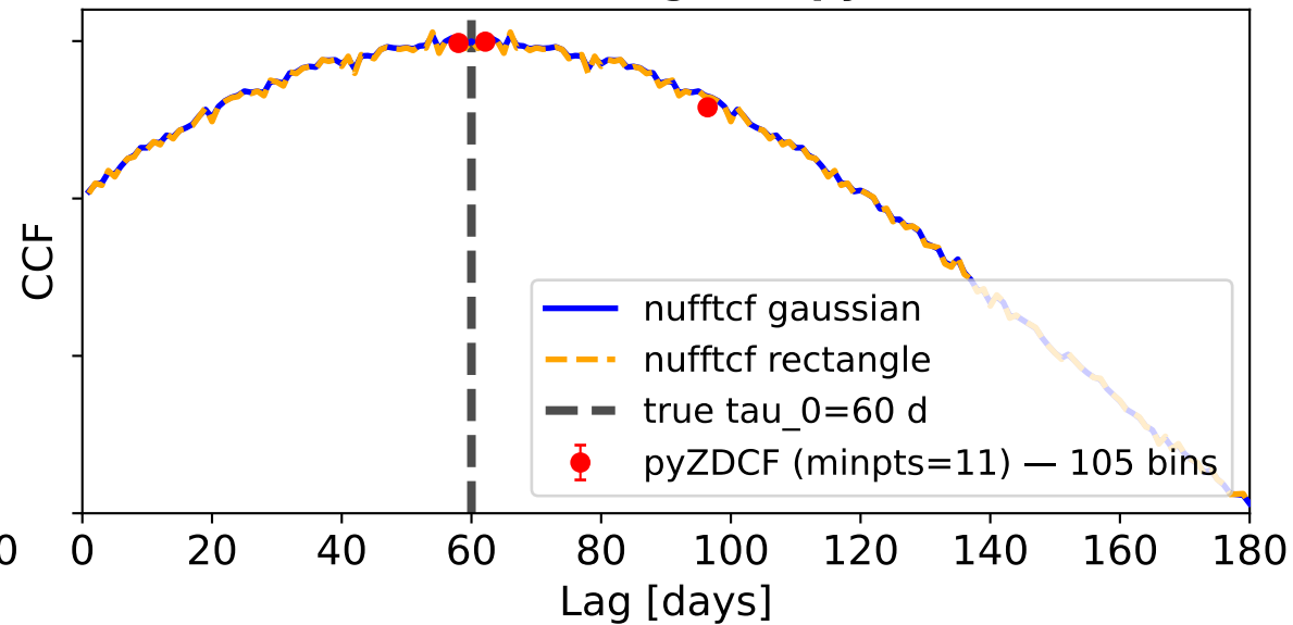
nufftcf rectangle vs pyZDCF
