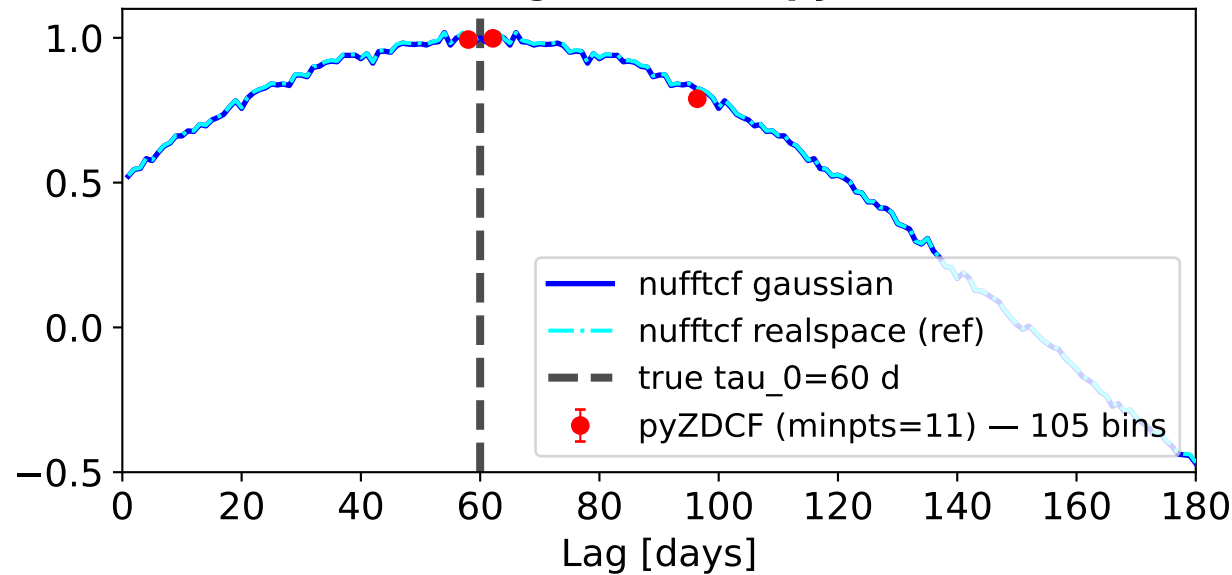
nufftcf gaussian vs pyZDCF
