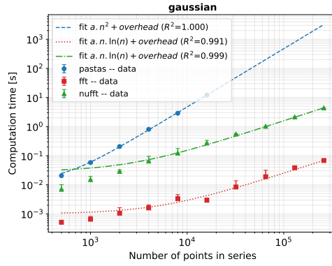
FIG. 9.— ACF benchmark on regularly-sampled data, pastas versus nufftcf (dedicated FFT path and general-purpose NUFFT path), gaussian kernel.
