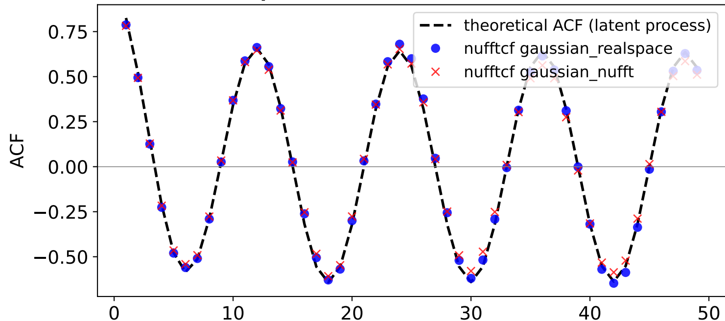
Recovered ACF (sparse data, heteroscedastic noise) vs true ACF
