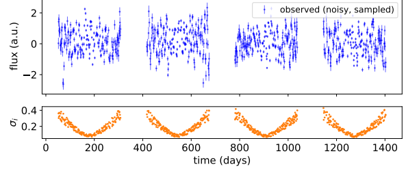
Figure 8: Simulated ground-based light curve (top; error bars show \sigma_i ) combining stellar-rotation modulation, correlated OU noise, seasonal/weather gaps, and heteroscedastic measurement noise (bottom).
