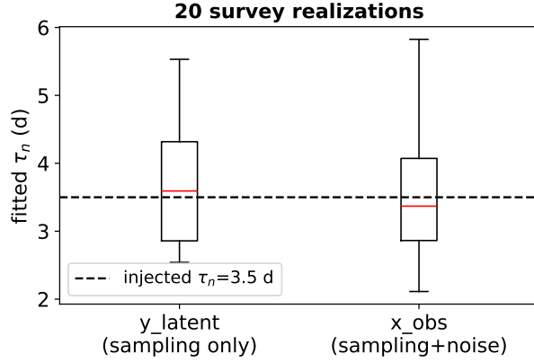
Figure 10: Fitted \tau_n over n_{mc} = 20 independent survey realizations, for the sampled-only latent signal and the sampled+noisy observed series, against the injected value (dashed). Medians are shown as red lines, box edges represent the first (Q1) and third (Q3) quartiles, and whiskers extend to the most extreme data point within 1.5 times the interquartile range (IQR) from the boxes.
