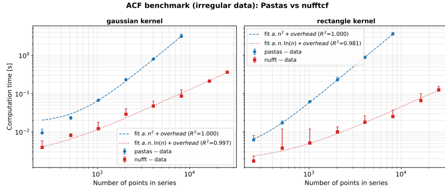
Figure 11: ACF benchmark, nufftcf versus pastas , on irregularly-sampled data (gaussian and rectangle kernels). Robust fit ( soft_l1 ); error bars show the min-to-max spread across repeats at each point.
