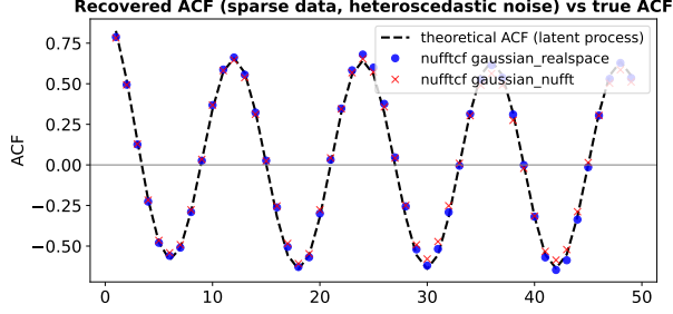
Figure 9: ACF recovered by nufftcf Gaussian real-space and NUFFT estimators from the sparse, heteroscedastic light curve of Figure 8, against the theoretical latent-process ACF (Equation 11).
