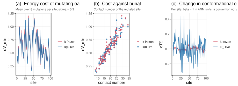
Figure 3. Blue = k_{ij}(l_{ij}) live, red = frozen. (a) \Delta V_{\min} per site. (b) The same against the mutated site’s contact number. (c) \Delta(TS) per site, \beta = 1 .
