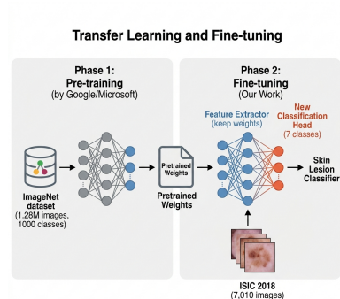
Figure: Transfer learning from ImageNet to ISIC: reuse generic features, replace only the classifier head.
