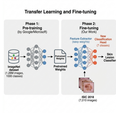
Figure: Transfer learning from ImageNet to ISIC: reuse generic features, replace only the classifier head.
