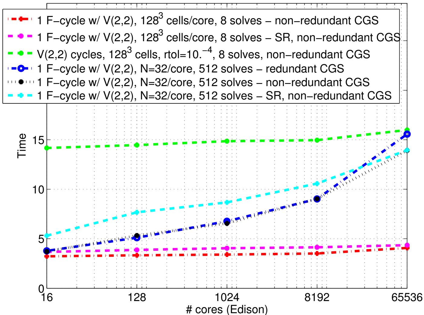
Solve times: Laplacian, u=(x^4 - L^2 x^2) , L=(2,1,1) (8 solves)
