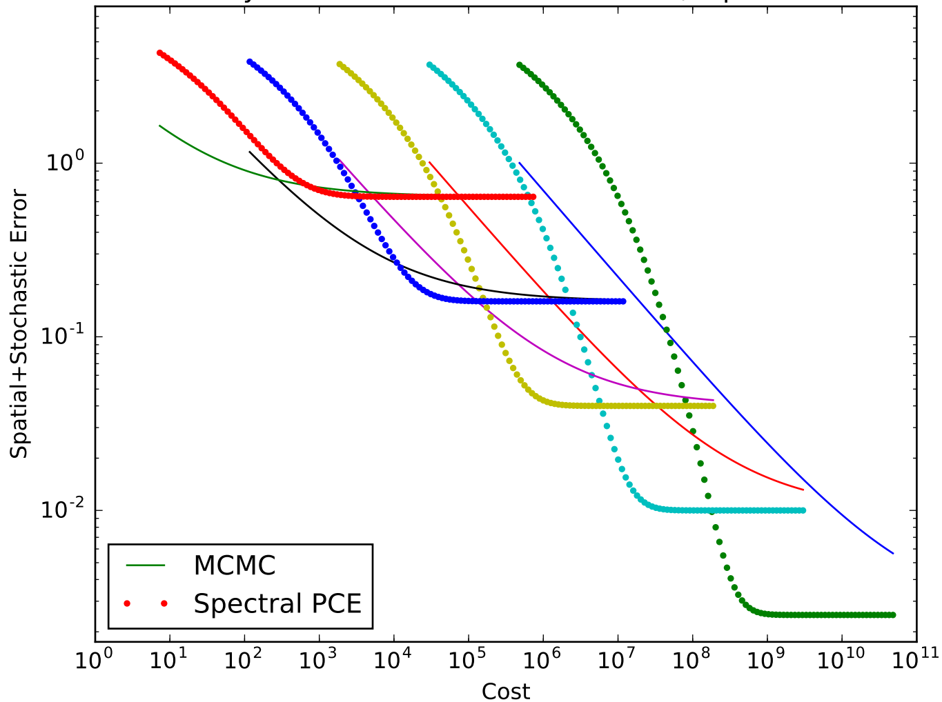
Accuracy-Cost Tradeoff for MCMC vs PCE, 3 parameters
