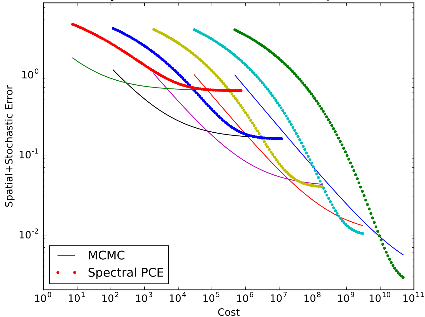
Accuracy-Cost Tradeoff for MCMC vs PCE, 5 parameters
