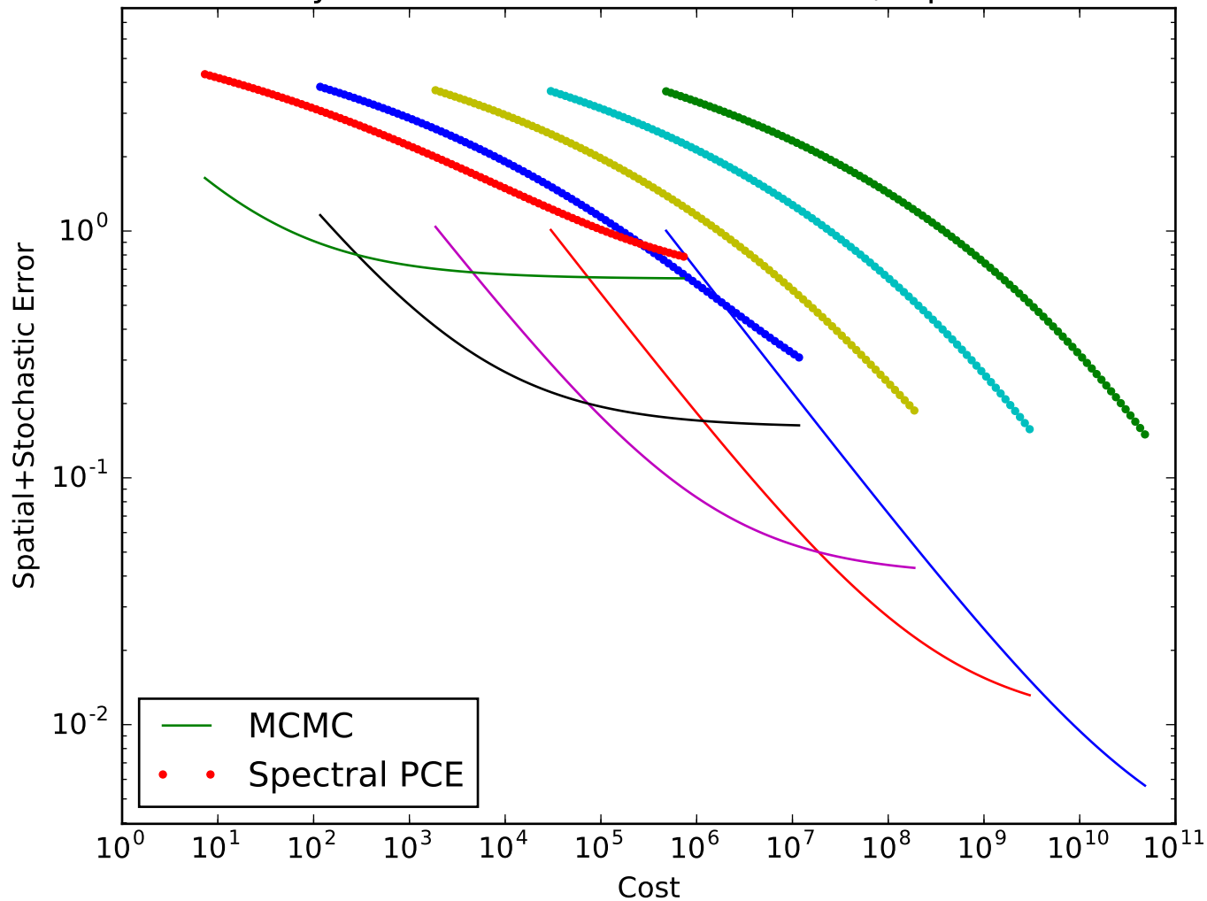
Accuracy-Cost Tradeoff for MCMC vs PCE, 8 parameters
