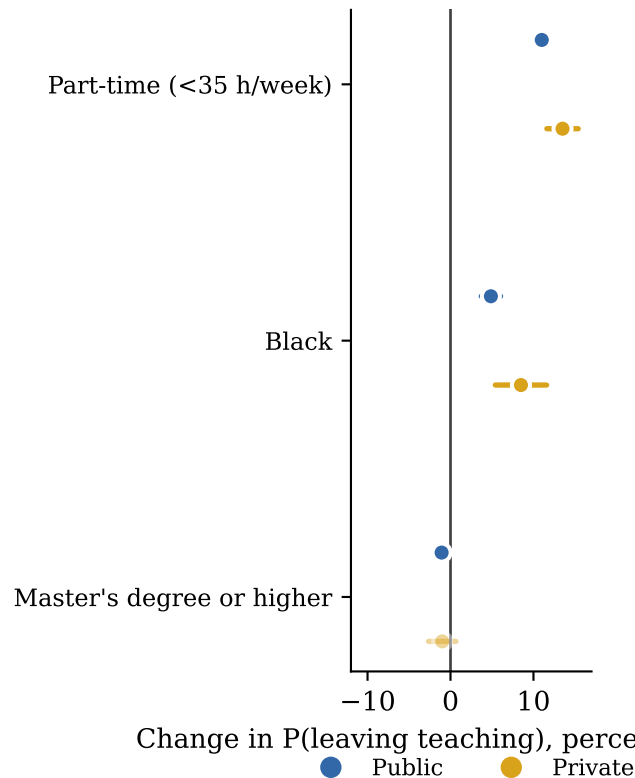
By sector
