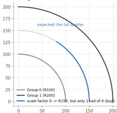
SC3: halfway between two arcs is an exact R150 arc
