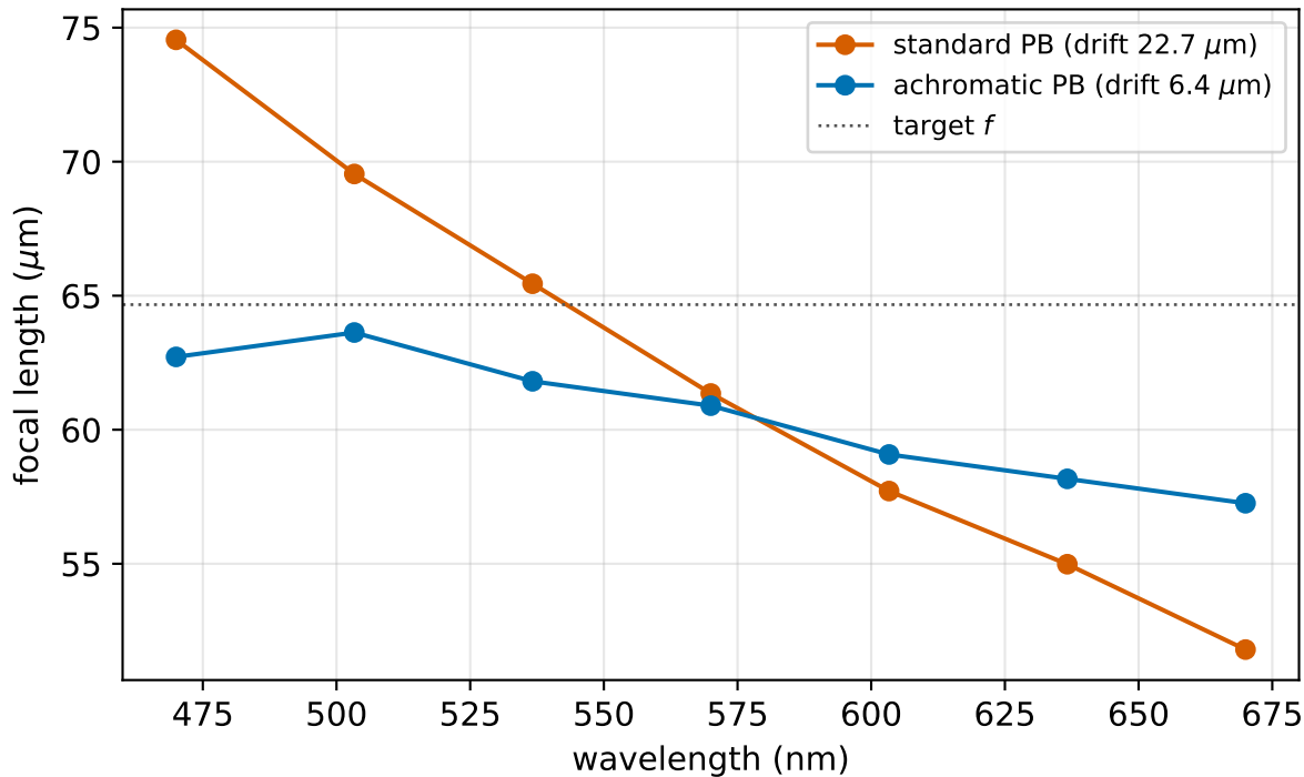
Chen-2018 achromat ( D=26.4\text{ }\mu\text{m} , f=64.7\text{ }\mu\text{m} , H=600\text{ nm} , 470-670 nm): single-etch group-delay engineering flattens the chromatic focal shift
