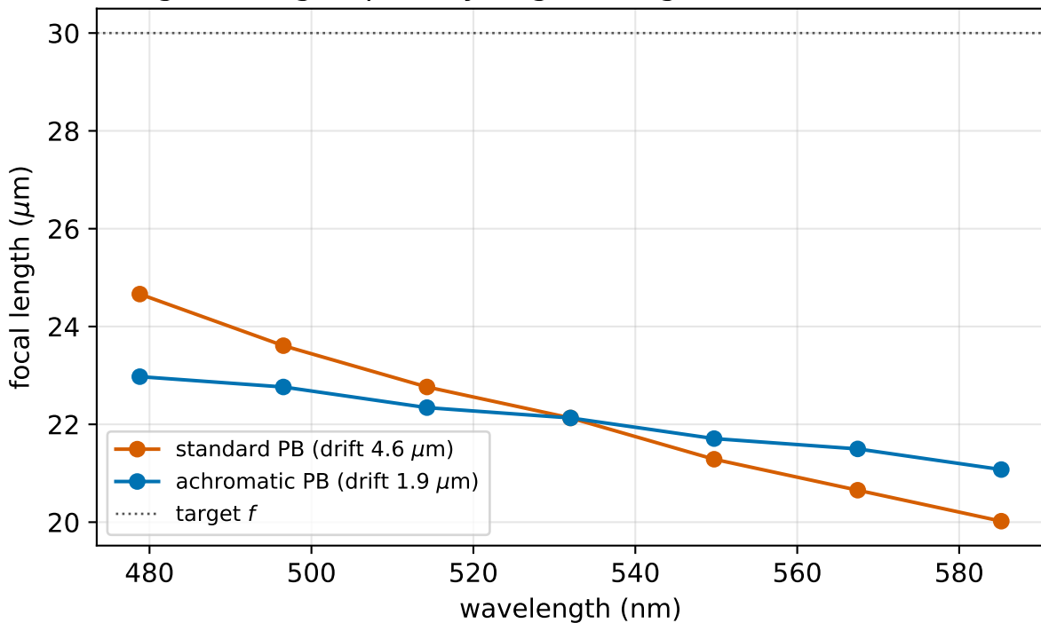
Broadband achromatic metalens (Chen 2018 recipe): single-etch group-delay engineering flattens the focal shift
