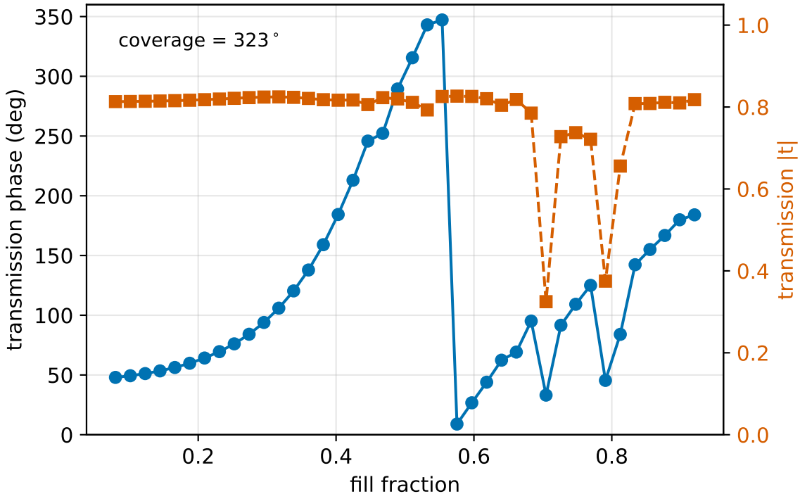
TiO 2 meta-atom library ( \lambda=532 nm, \Lambda=350 nm)
