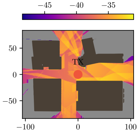
(a) Ground truth G_{GT} (dB) (small scene).
