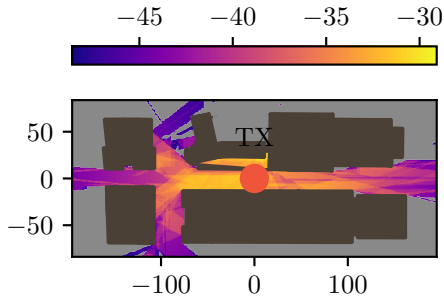
(c) Ground truth G_{GT} (dB) (medium scene).
