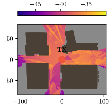
(b) Prediction G_{pred} (dB) (small scene).
