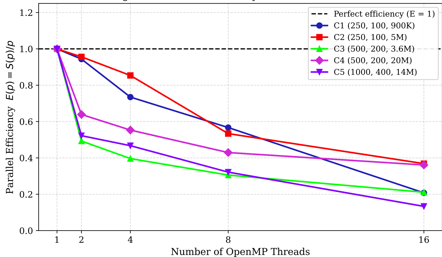
Figure 4: Parallel Efficiency vs. Number of Cores
