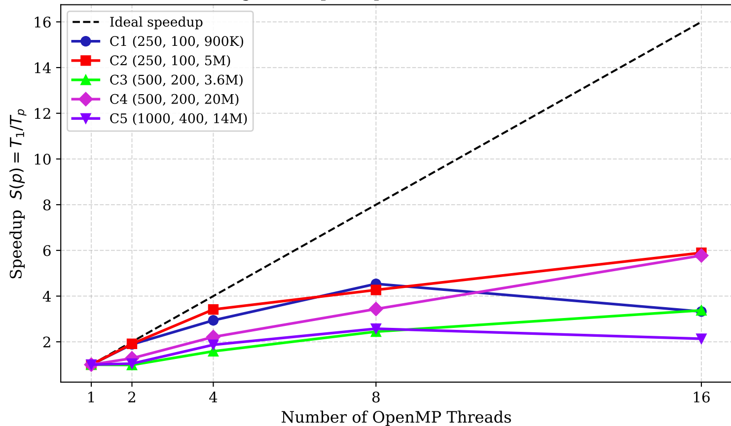
Figure 3: Speedup vs. Number of Cores
