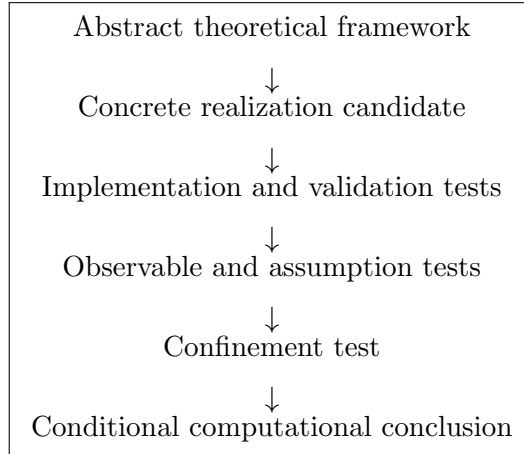
Figure 1: Realization hierarchy for the computational project. The abstract framework is instantiated by a concrete TN or QEC realization, which must first pass implementation and validation tests. Only then are the relevant structural observables and realization-dependent assumptions evaluated. Only after these conditions have been satisfied is the confinement prediction tested.
