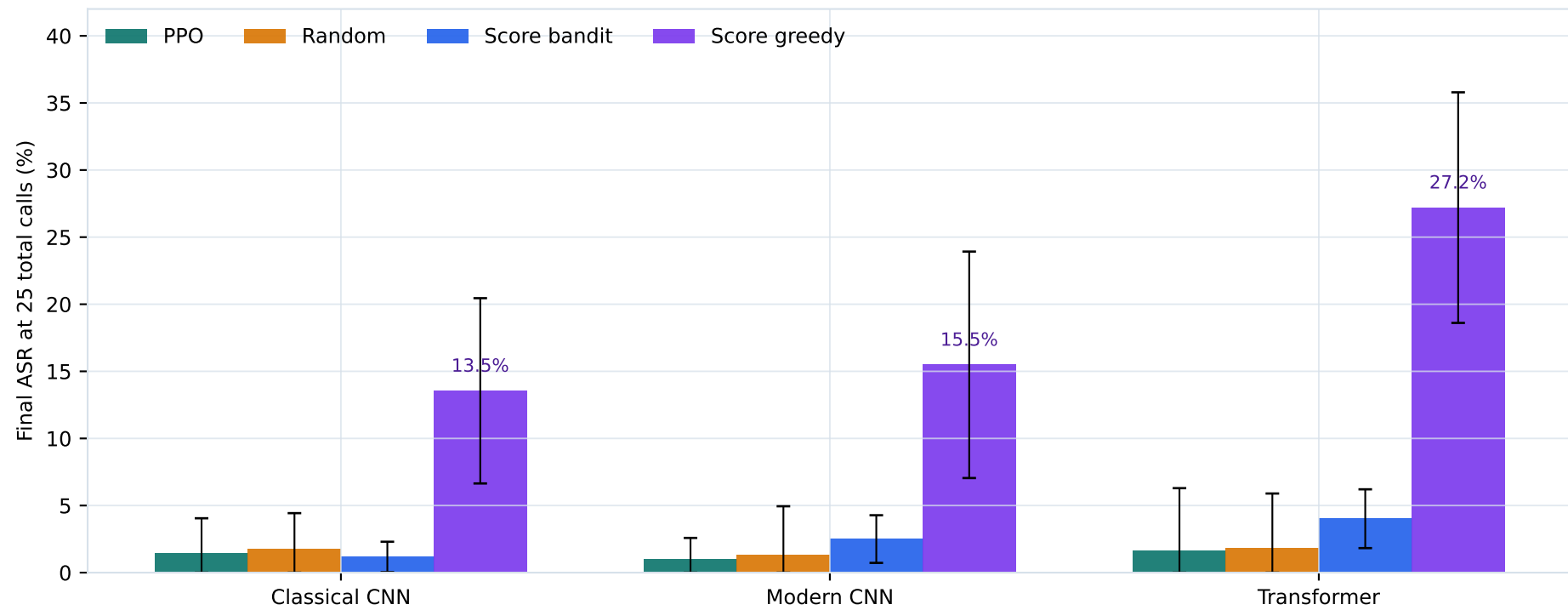
Frozen attack success on held-out victim families
