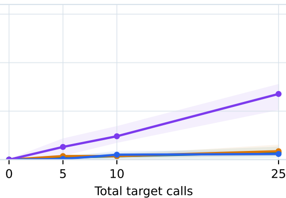
Classical CNN
