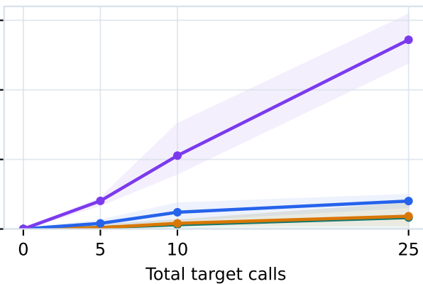
Transformer
