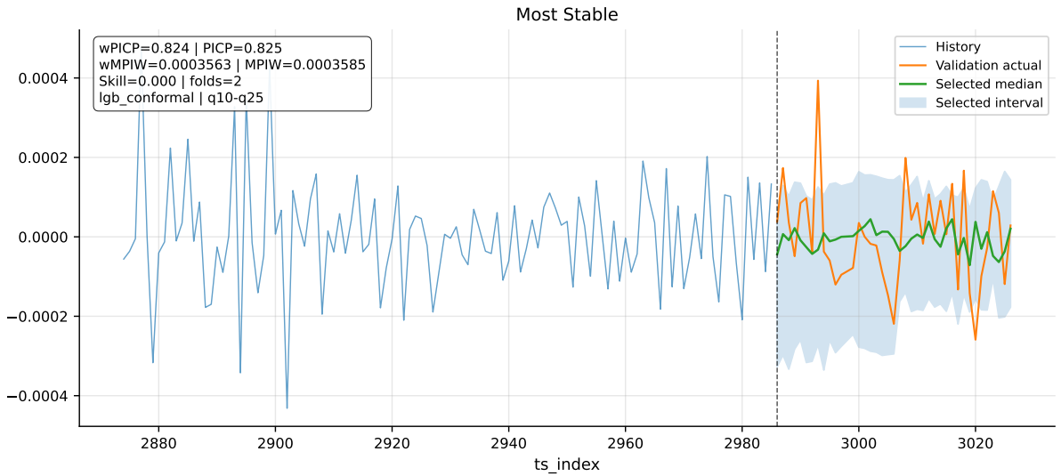
Figure 33: Most-stable series. The series itself is near-flat at scale 10^{-4} , so the median forecast carries no signal; the calibrated band still covers most observations (wPICP 0.82), which is the correct behaviour: the interval acknowledges its own uncertainty rather than committing to a confident wrong point estimate.
