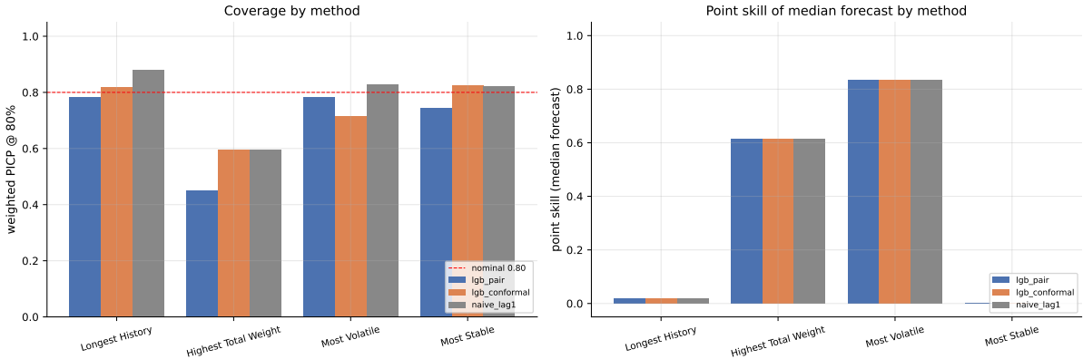
Figure 27: Method comparison across the four representative series. Left: weighted PICP at the nominal 80% target (red dashed line). Right: skill of the LightGBM median forecast (the median is identical across all three methods, so the right panel reads as the underlying point-forecast skill on the validation segment).
