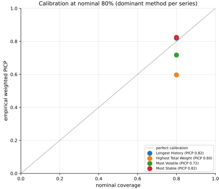
Figure 28: Empirical weighted PICP versus the nominal 80% target, one point per series for the dominant method. Diagonal dashed line is perfect calibration. The longest-history and most-stable series sit very close to the diagonal; the most-volatile and highest-weight series under-cover slightly.
