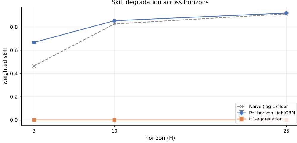
Figure 35: Weighted skill across horizons under each strategy. Per-horizon LightGBM (blue) tracks the rising Naive floor (grey dashed) and beats it at every horizon. H1-aggregation (orange) is flat at zero across all horizons.
