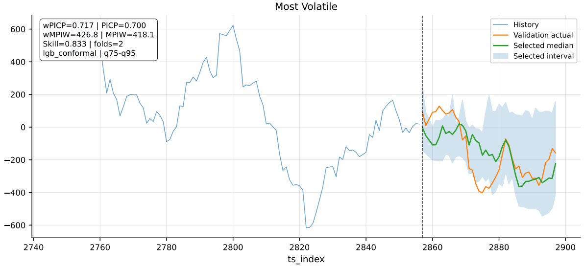
Figure 32: Most-volatile series. The headline visual of the chapter: median forecast tracks the validation trajectory closely (skill 0.83), the calibrated band hugs the truth, and weighted PICP is 0.72 on a 40-row validation segment.
