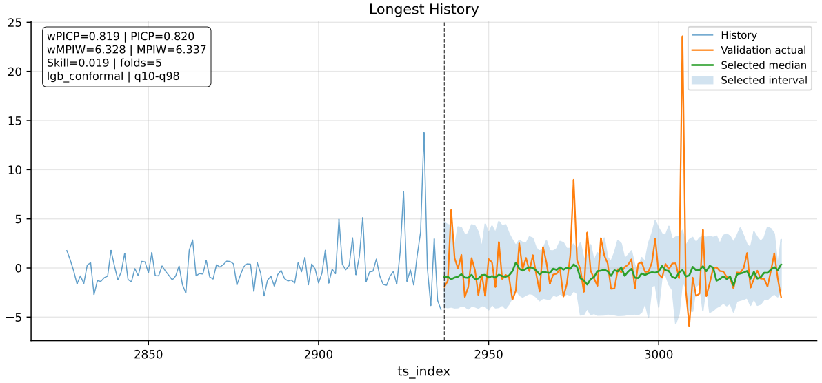
Figure 30: Longest-history series. Coverage is well-calibrated (wPICP 0.82); point skill is near zero, which is honest — the data has no exploitable feature signal at this resolution.
