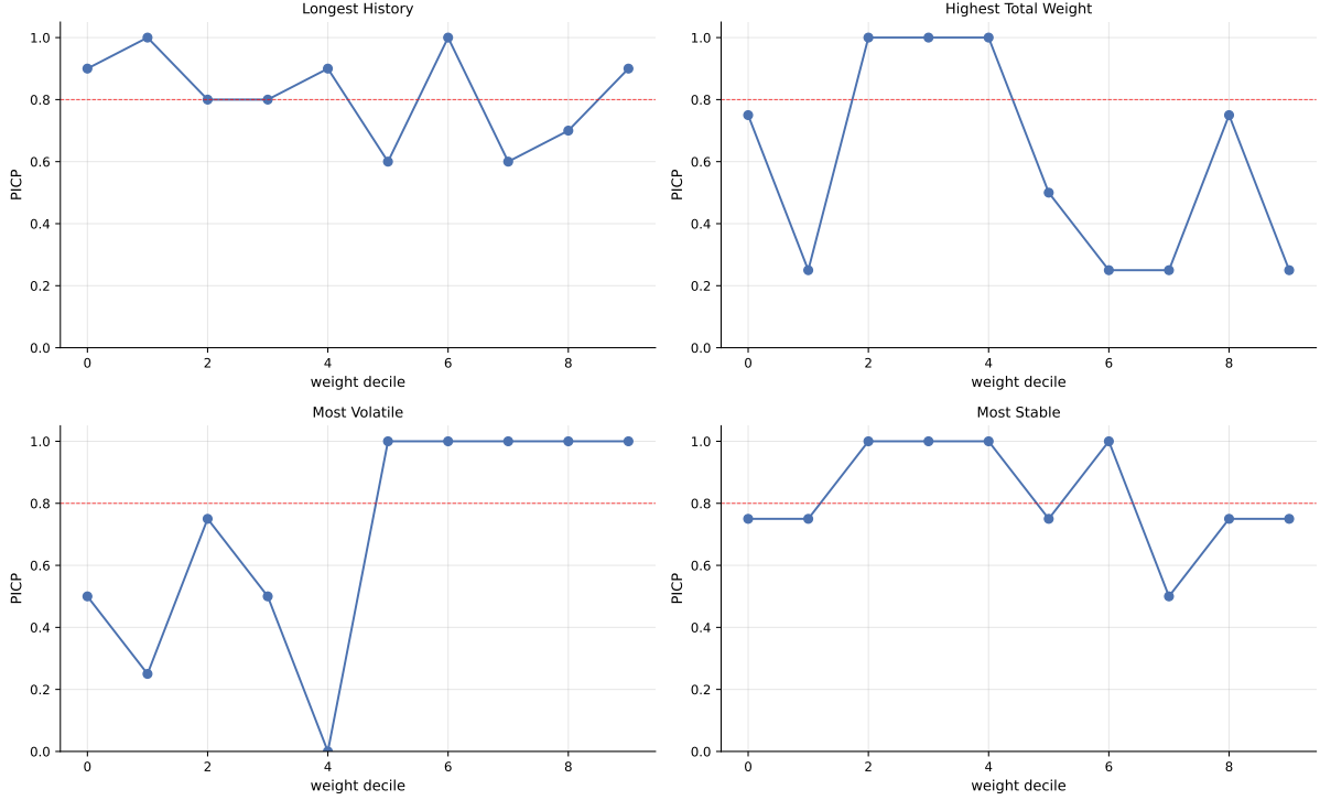
Figure 29: Empirical PICP by weight decile, one panel per series. Red dashed line is the nominal 80% target. The validation segments are small ( n = 40\text{--}100 ) so per-decile estimates are noisy, but the trend across deciles indicates whether high-weight rows receive comparable coverage to low-weight rows.
