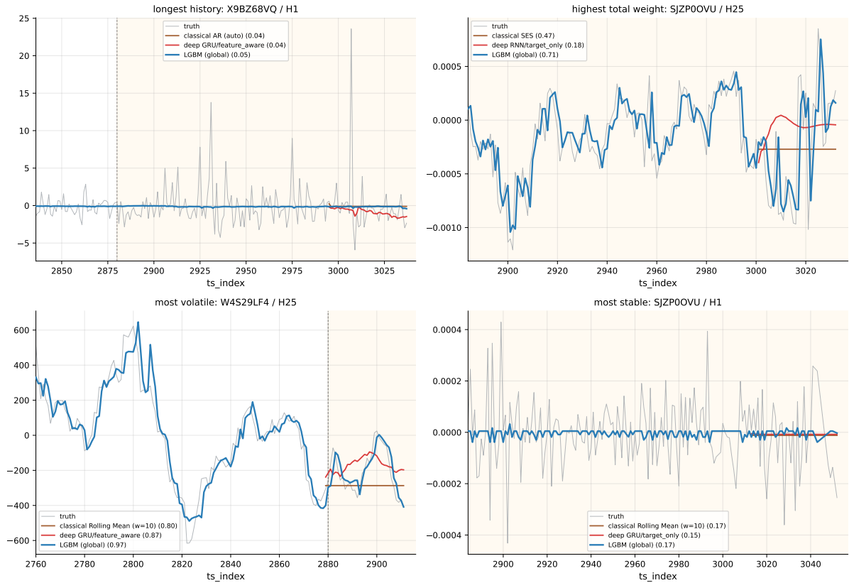
Figure 25: Predictions of global LightGBM (vivid blue), the best classical model from Section 5 (brown), and the best deep configuration from Section 6 (red), overlaid on the four representative series. Truth is the thin grey line. The light orange band marks the post-cutoff region. Vertical dashed line: canonical train/validation cutoff. Skill values in the legend are weighted skill scores on the post-cutoff segment available for each model.
