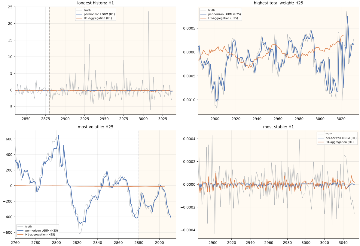
Figure 36: Forecast overlays on the four representative series at their native horizons. Truth in muted grey, per-horizon LightGBM in blue, H1-aggregation in orange. The orange line stays close to zero on every panel, while the blue line tracks the truth where signal is available.
