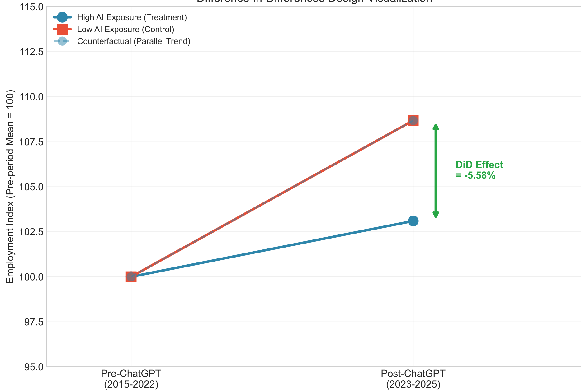
Difference-in-Differences Design Visualization
