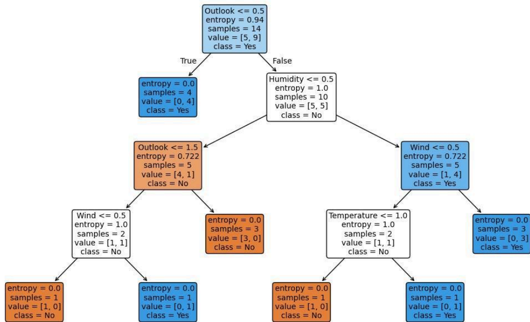
Decision Tree using ID3 Algorithm
