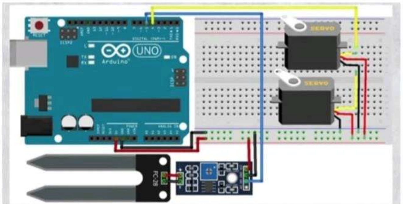
Figure 4.4.1: Schematic Diagram of the Circuit
