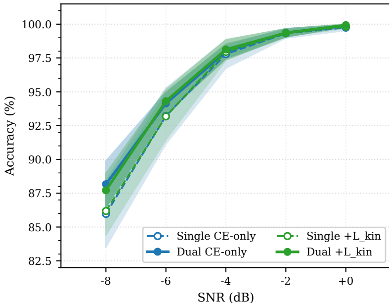
(a) Single vs Dual Sensor — Accuracy vs SNR (n=8 @ -4/-6/-8dB)
