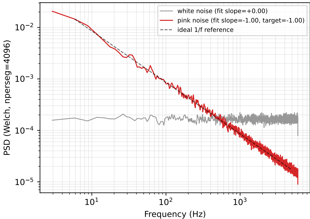
Pink vs white noise PSD — spectral verification (bearmamba3.noise)
