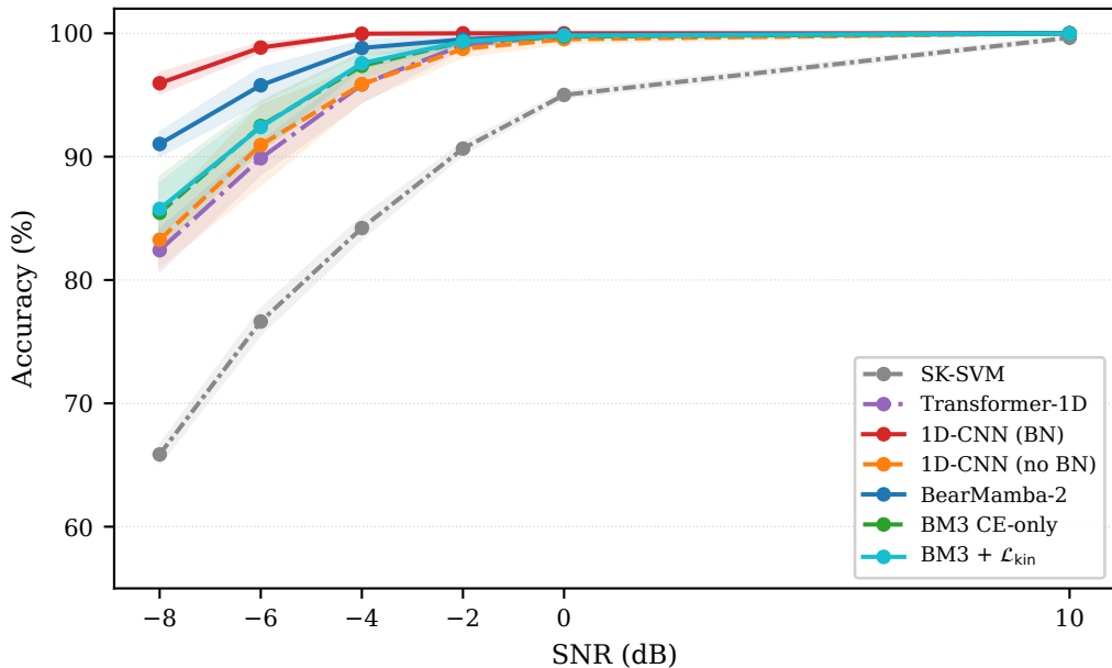
CWRU 4-class: all baselines ( \pm 1\sigma , 5 seeds)
