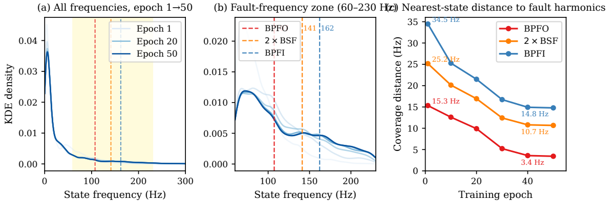
Fig. 3. II frequency snapshot: BearMamba-3 / CWRU SNR=0 dB / \mathcal{L}_{\text{kin}} ( \lambda = 0.01 , cover), 5 seeds (640 samples/epoch). (a) KDE of all time-averaged state frequencies \bar{f}_{h,k} in 0–300 Hz at epochs 1 (lightest) through 50 (darkest blue); yellow band marks the 60–230 Hz fault-frequency zone. (b) Zoomed KDE in the fault-frequency zone; dashed lines mark BPFO (107.4 Hz), 2 \times \text{BSF} (141.2 Hz), BPFI (162.2 Hz). (c) Mean nearest-state coverage distance vs epoch: BPFO 15.3 \rightarrow 3.4 Hz (4.5 \times ); BPFI 34.5 \rightarrow 14.8 Hz (2.3 \times ).
