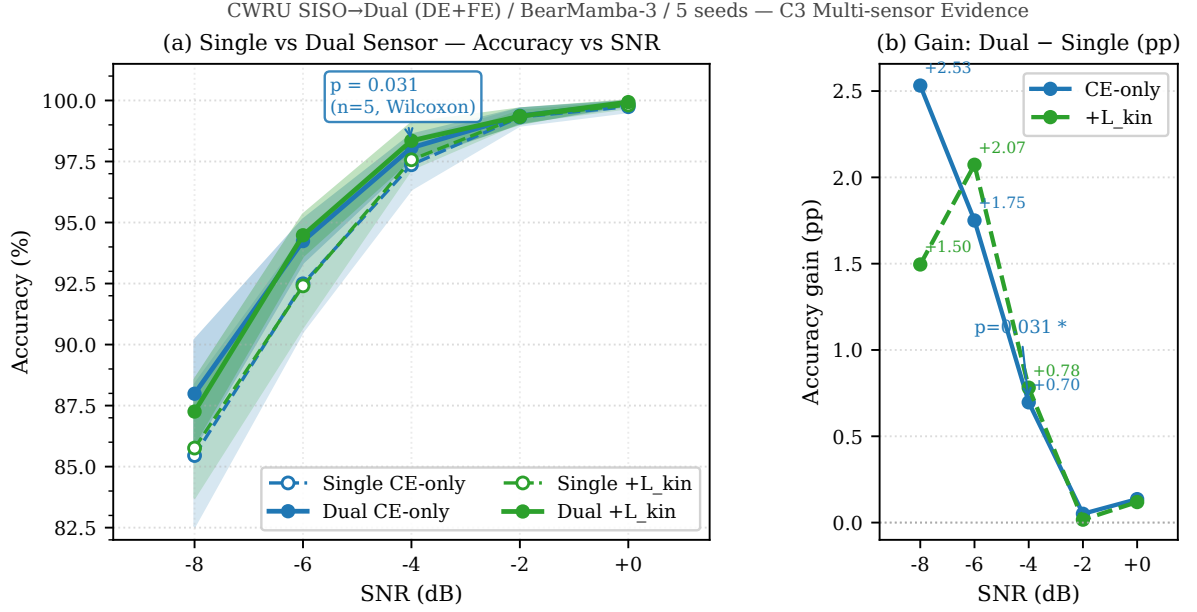
Fig. 7. CWRU single vs dual (DE+FE) sensor accuracy vs SNR ( \pm 1\sigma shaded, 5 seeds). (a) Accuracy curves: solid = dual, dashed = single, blue = CE-only, green = +L_{\text{kin}} . Annotation marks the unique statistically significant point: -4 dB nokin Wilcoxon p = 0.031 ( n = 5 , one-sided). (b) Gain (dual – single) in percentage points; gain is positive at all SNR values, peaking at -8 dB ( +2.5 pp).
