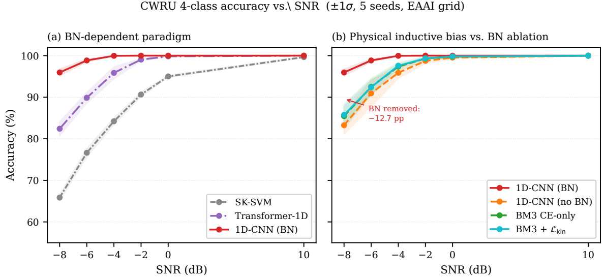
Fig. 8. CWRU 4-class accuracy vs. SNR ( \pm 1\sigma , 5 seeds, EAAI evaluation grid). (a) BN-dependent paradigm: SK-SVM, Transformer-1D, and 1D-CNN all rely on BatchNorm or manually designed features for low-SNR stability; performance drops sharply beyond -6 dB for non-CNN methods. (b) BN ablation on 1D-CNN (Phase 2b): removing all eight BatchNorm layers reduces 1D-CNN from 95.96% to 83.26% at -8 dB ( \Delta = -12.69 pp); BM3 CE-only (85.45%) and BM3 + \mathcal{L}_{\text{kin}} (85.76%) overlap the no-BN CNN curve ( p = 0.125 ), confirming that BatchNorm is the principal source of 1D-CNN’s within-condition advantage over BM3.
