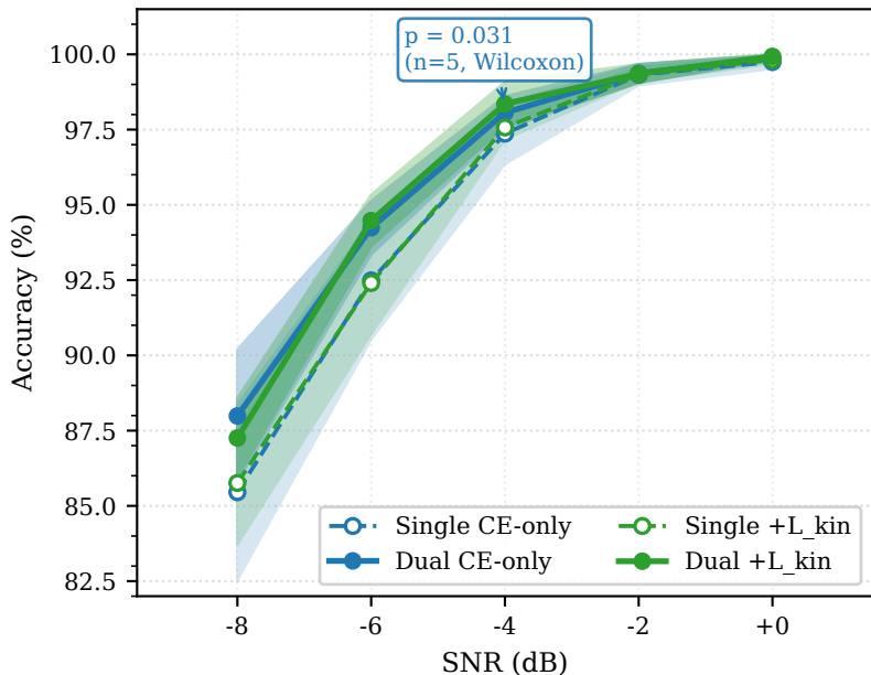
(a) Single vs Dual Sensor — Accuracy vs SNR
