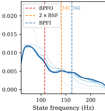
(b) Fault-frequency zone (60–230 Hz)
