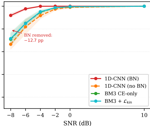
(b) Physical inductive bias vs. BN ablation
